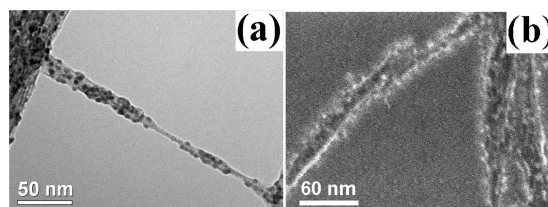
Figure 1. (a) TEM and (b) SEM images of HiPCO SWNTs decorated by 3.5 nm CdSe nanoparticles.
