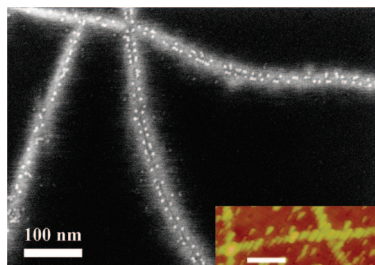
Figure 3. SEM image of SWNTs, grown on a SiO 2 /Si substrate by CVD, decorated by 3.5 nm CdSe nanoparticles, with AFM inset. The scale bar in the inset is 100 nm.
