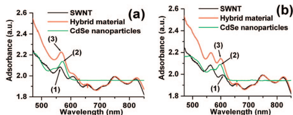
Figure 2. (a) UV–vis adsorption of HiPCO SWNTs, 3.6 nm CdSe nanoparticles, and the corresponding hybrid material. Peak (1) is the SWNT transition peak at 562 nm. Peak (2) is the first exciton peak of CdSe nanoparticles at 571 nm. These peaks contribute to the adsorption maximum at 568 nm [peak (3)] for the hybrid material. (b) UV–vis adsorption of HiPCO SWNTs, 4.5 nm CdSe nanoparticles, and the corresponding hybrid material, with the peaks at 598 nm, 607 nm, 600 nm, respectively. The vertical scales differ for each curve. All samples are measured in pyridine.
