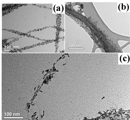
Figure 4. TEM images of HiPCO SWNTs decorated by different CdSe nanoparticles: (a) 6.6 nm diameter CdSe nanoparticles; (b) ZnS shell, 3.5 nm diameter CdSe core nanoparticles; (c) CdSe nanorods, 4.5 nm in diameter by 16 nm in length.
